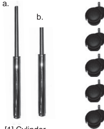
B. [1] Cylinder [a] 91-02606 model C. [5] Castors [b] 91-02609 model
